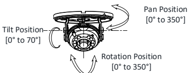
Figure 2-16 3-Axis Adjustment
