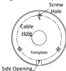
Figure 2-1 Drill Template
