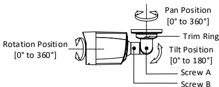
Figure 2-6 3-Axis Adjustment
