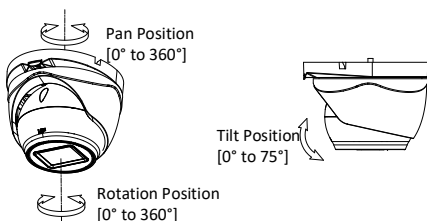
Figure 2-12 3-axis Adjustment
