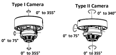
Figure 2-4 3-Axis Adjustment
