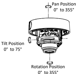
Figure 2-10 3-Axis Adjustment
