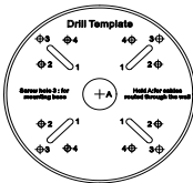
Figure 2-1 The Drill Template
