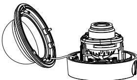
Figure 2-8 Remove the Bubble and the Black Liner
