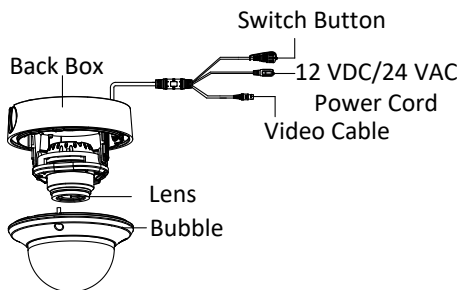
Figure 1-3 Overview of Type I Camera
