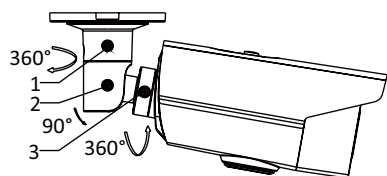
Figure 2-4 3-axis Adjustment
