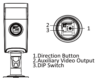
Figure 2-3 Image Adjustment
