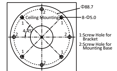
Figure 2-1 Drill Template
