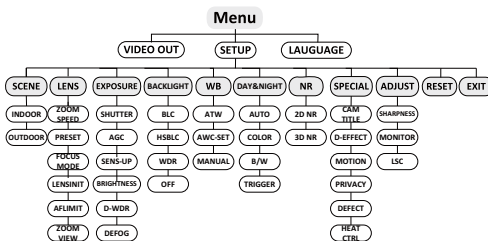
Figure 3-1 Main Menu
