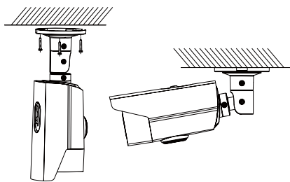
Figure 2-2 Fix the Camera to the Ceiling
