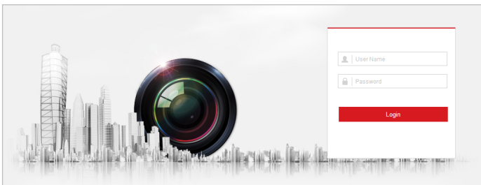
Figure 4-1 Login Interface
