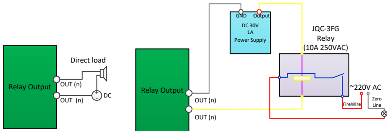
Figure 1-8 Alarm Output
