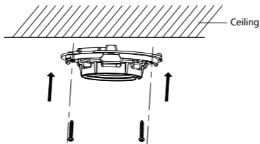
Figure 2-12 Secure the Camera to the Ceiling
