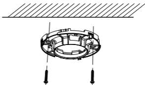
Figure 2-19 Install the Mounting Base
