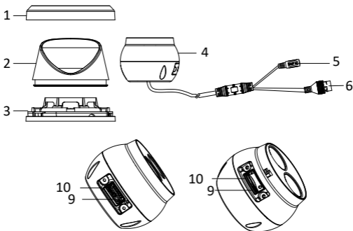
Figure 1-4 Type IV Turret Camera
