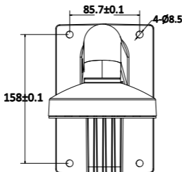
Figure 2-36 Dimension of Demonstrated Wall Mounting Bracket
