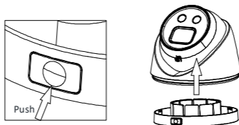
Figure 2-30 Remove the Bottom Base
