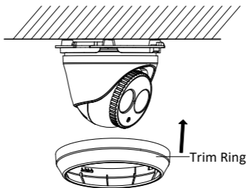
Figure 2-8 Install the Trim Ring
