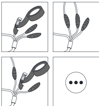
Figure 2-44 Waterproof Cables
