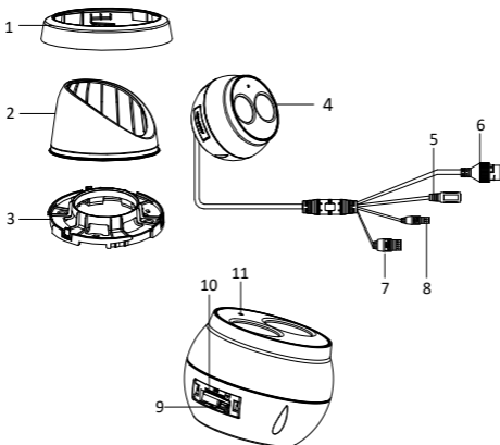
Figure 1-3 Overview of Type III Turret Camera
