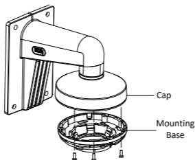
Figure 2-37 Fix Mounting Base
