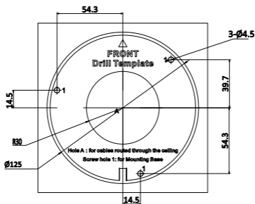
Figure 2-25 Drill Template
