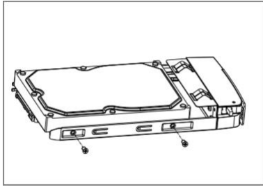
Figure 2-7 Fix HDD
