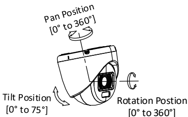
Figure 2-15 3-Axis Adjustment
